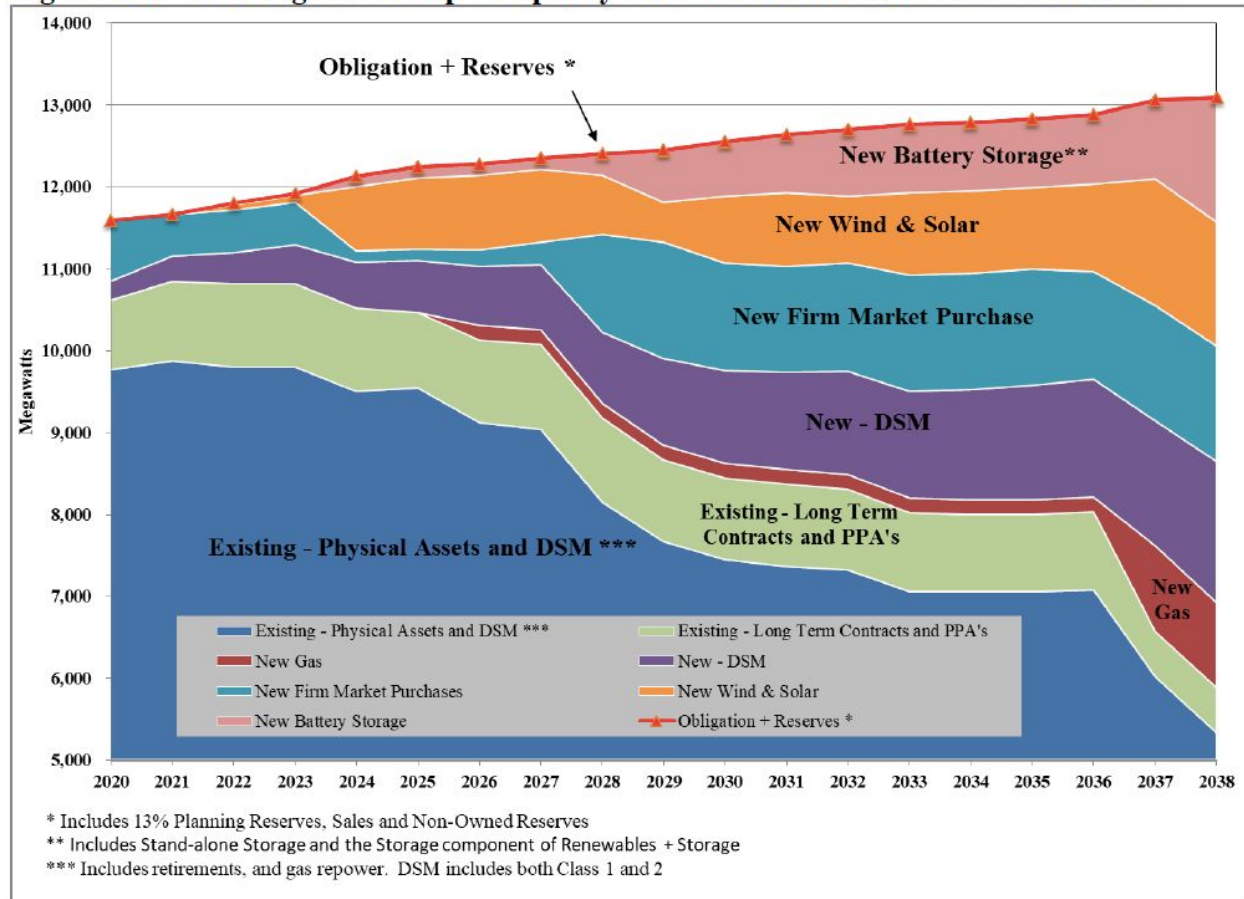
Figure 1: Meeting PacifiCorp’s Capacity Needs with Preferred Portfolio Resources from PacifiCorp 2019 Integrated Resource Plan at 256.
